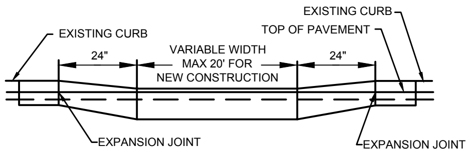
ELEVATION VIEW
