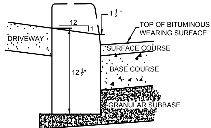
SECTION DETAIL
