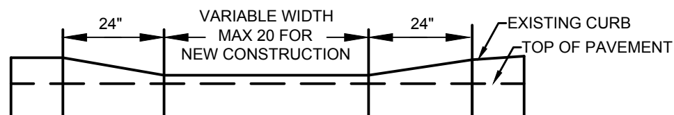
ELEVATION VIEW
