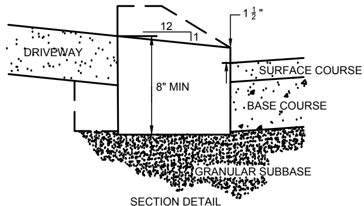
SECTION DETAIL
